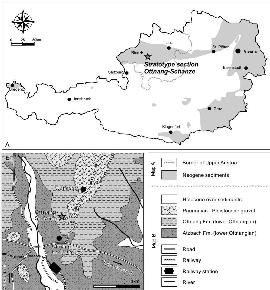
Fig. 2. (A) Location of the stratotype section within the Austrian NAFB. (B) Geography and geology of the study area based on Krenmayr and Schnabel (2006) and Rupp et al. (2008).
