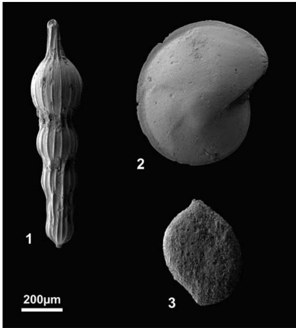
Plate 1. Biostratigraphic marker species of benthic foraminifers. 1: Amphicoryna ottnangensis (Toula); Sample OS 11. 2: Lenticulina inornata (D'Orbigny); Sample OS 11. 3: Sigmoidolopsis ottnangensis Cicha, Ctyroka & Zapletalova; Sample OS 24.
