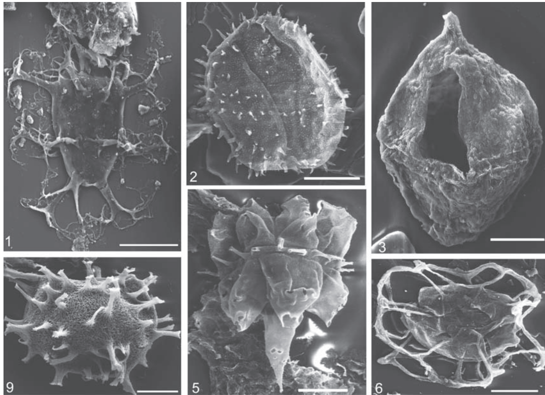
Plate 3. Biostratigraphic marker species of dinoflagellate cysts. Scale bar = 20 \mu\text{m}
