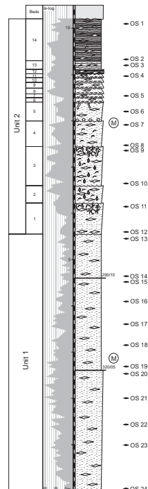
Fig. 1. Log of the stratotype section Otnnang-Schanze and range chart for biostratigraphically relevant species of benthic foraminifers, dinoflagellate cysts and calcareous nannoplankton as revealed in this study. See text for discussion.
