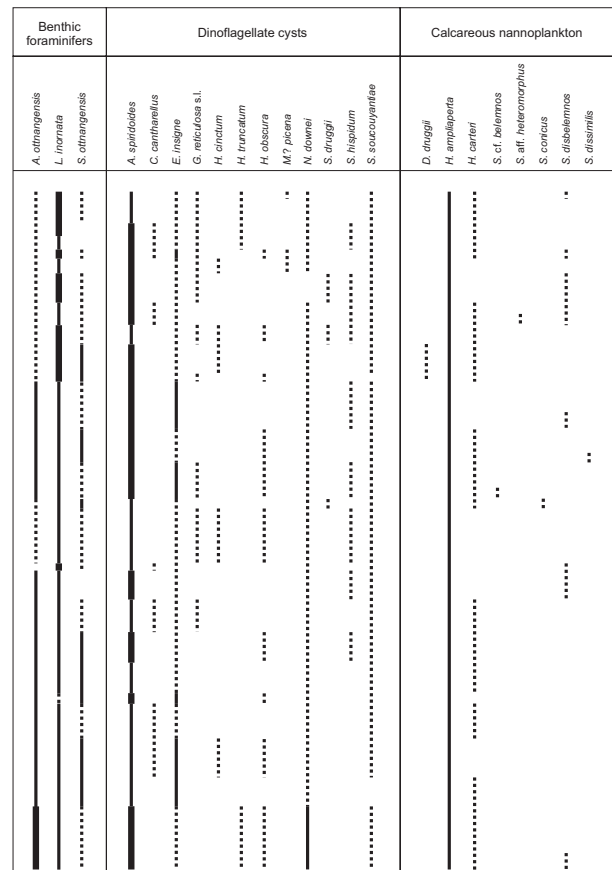
Fig. 1. Log of the stratotype section Otnnang-Schanze and range chart for biostratigraphically relevant species of benthic foraminifers, dinoflagellate cysts and calcareous nannoplankton as revealed in this study. See text for discussion.
